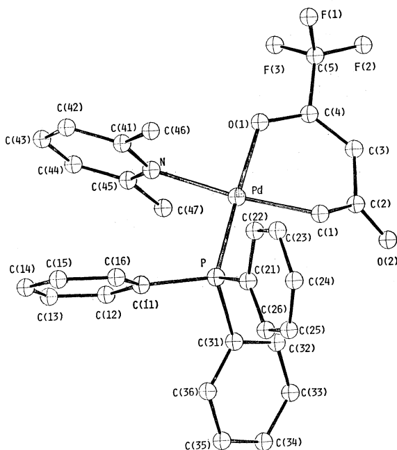
Fig. 3. The numbering scheme of non-hydrogen atoms of the 5 molecule.
